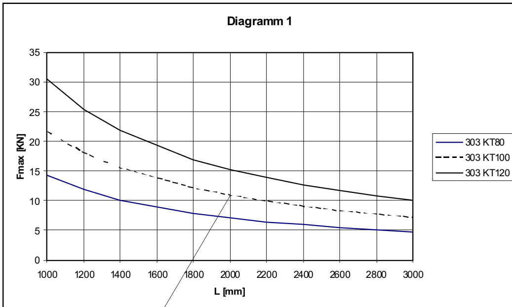
Diagramm 1 : Point loading (middle) for angle consoles at static load
