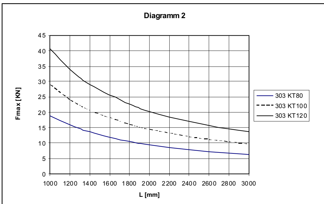
Diagramm 2 : Point loading (middle) for detached bridge at static load
